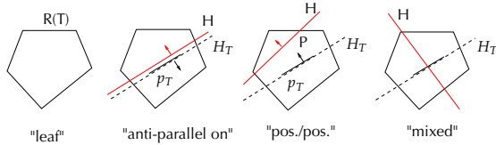
Figure 29: The main building block of the algorithm consists of these four cases (plus analogous ones).
