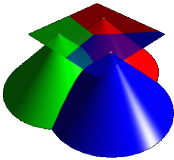
Figure 62: The distance function of a point site in the plane is a cone. 44
