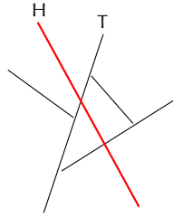
Figure 28: The fundamental step of the construction is this simple operation, which merges a BSP and a plane.
