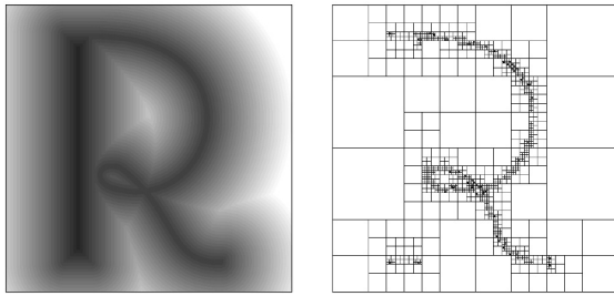
Figure 60: Representing distance fields by octrees has both memory and computational advantages.
