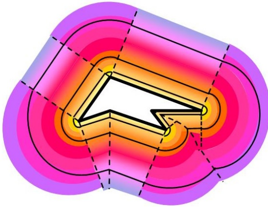
Figure 56: Example of a distance field in the plane for a simple polygon (thick black lines). The distance field inside the polygon is not shown. The dashed lines show the Voronoi diagram for the same polygon. The thin lines show isosurfaces for various isovalues.
