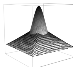
Figure 6.4: Projections and its comparisons to the function of figure 6.3, shown upside down.
