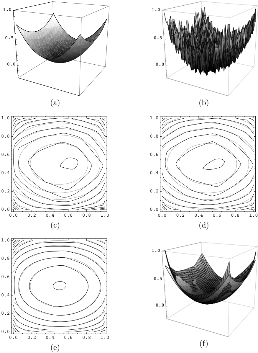
Figure 6.6: Fitting a convex surface to perturbed data. Original function (a), perturbed data (b), level curves of the L^1 projection (c), level curves of the L^2 projection (d), level curves of the L^\infty projection (e), 3D graphs of the unperturbed function and L^\infty projection (f).
