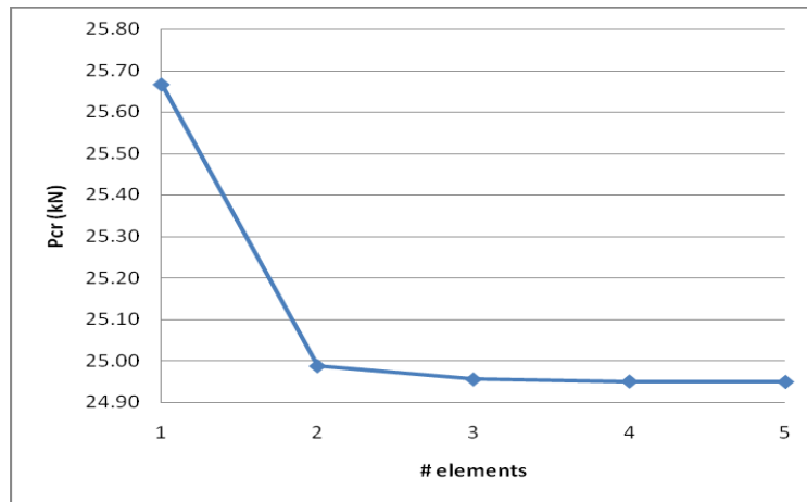
Figure 5 – Critical loads versus number of elements (ABAQUS) – Plane 1.
