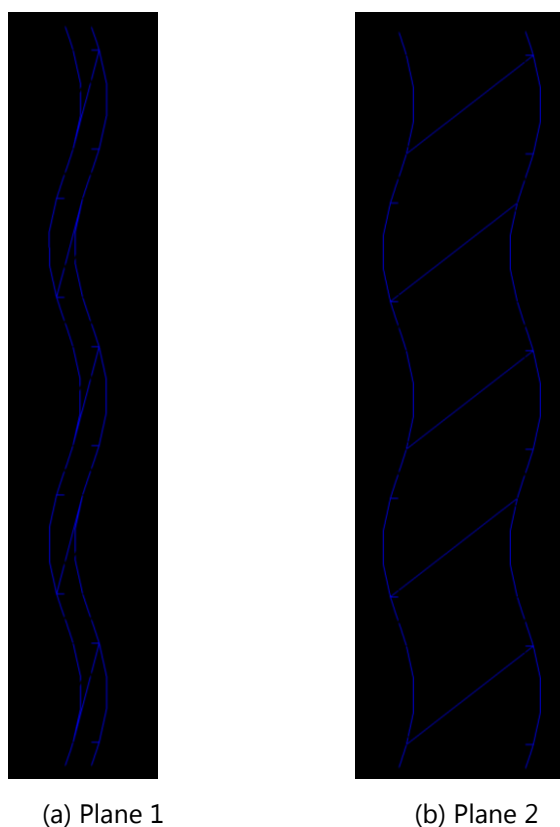
Figure 7 – Buckling modes of Example 1.
