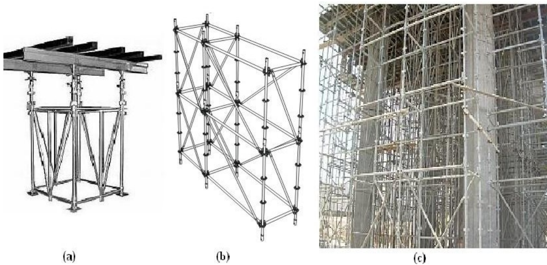
Figure 3 – Assembled steel scaffolding.
