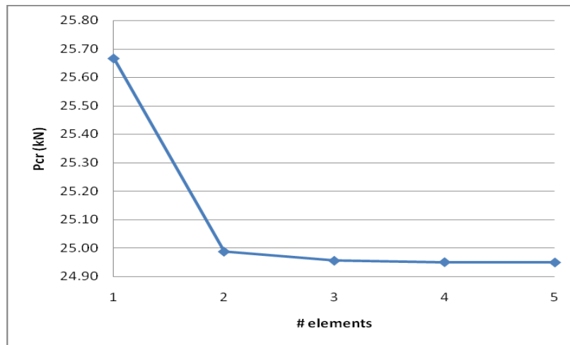
Figure 6 – Critical loads versus number of elements (ABAQUS) – Plane 2.
