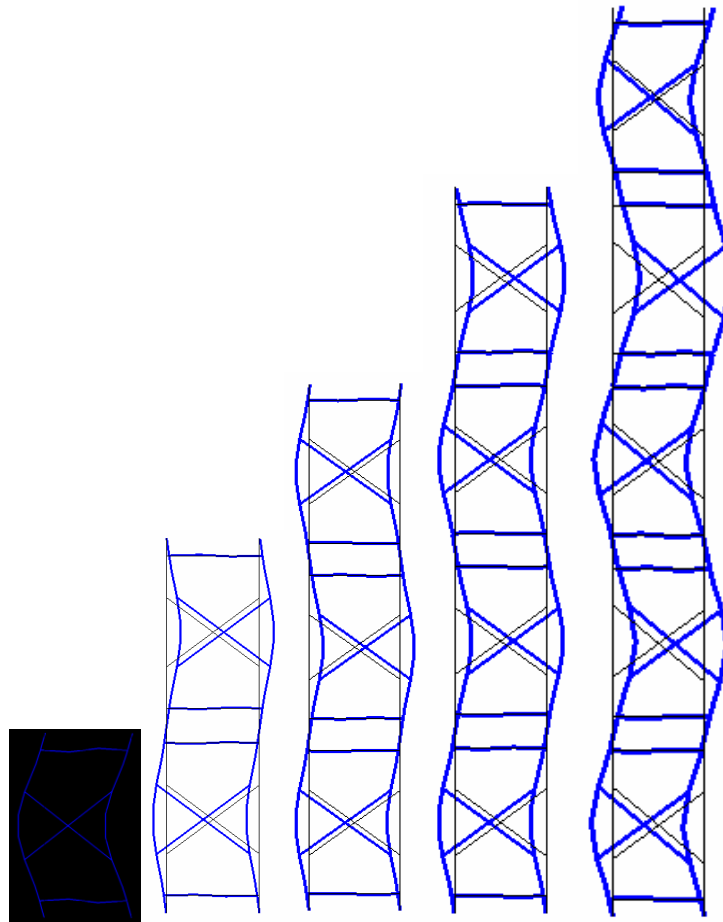
Figure 9 - Buckling modes of Example 2 – Plane 2.
