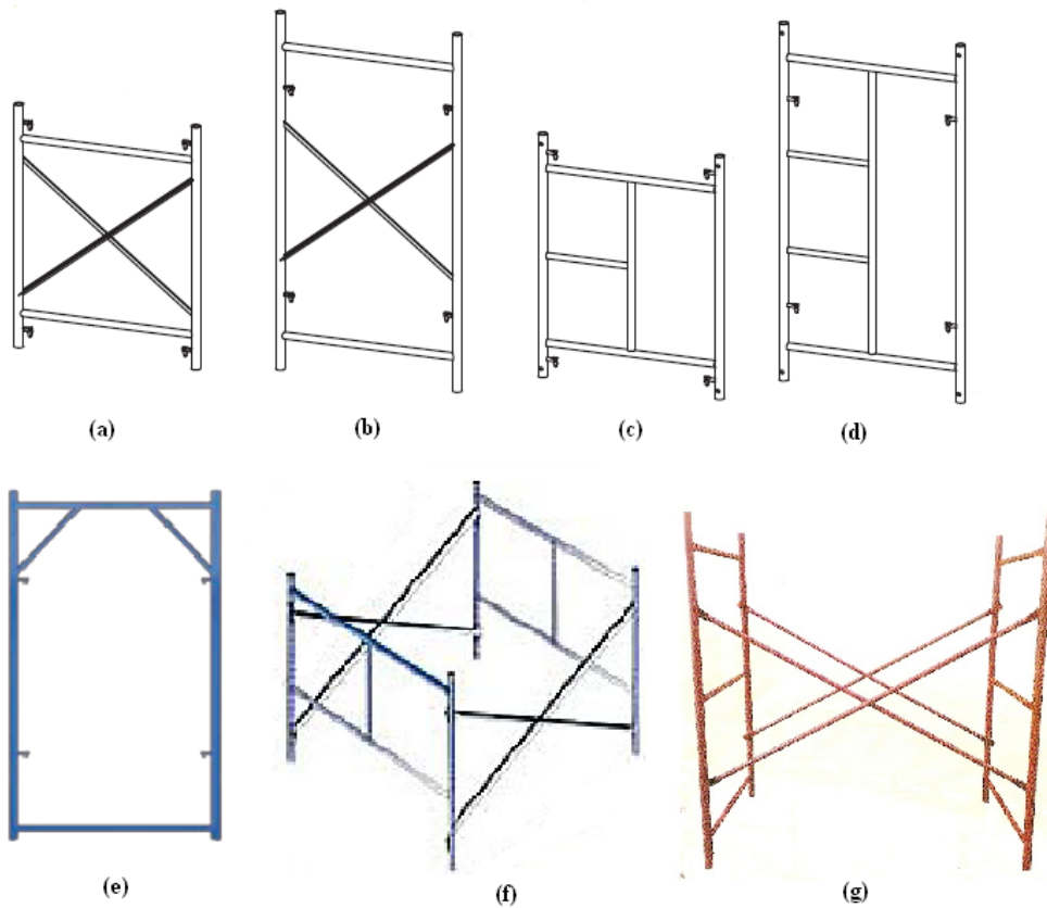
Figure 2 – Welded steel frames.
