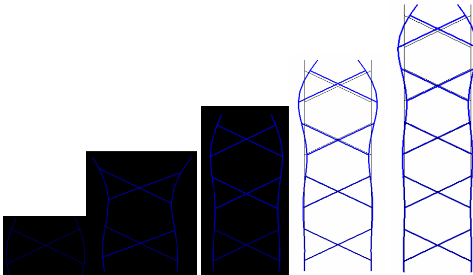
Figure 8 – Buckling modes of Example 2 – Plane 1.
