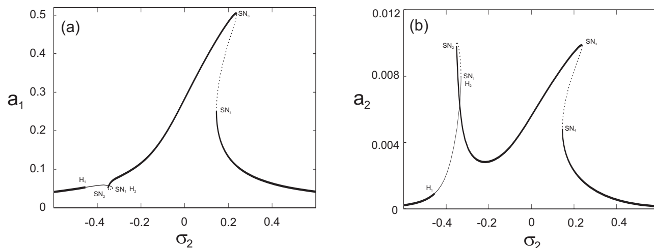
Figure 4. Frequency-response curves for: (a) first and (b) second modes, when f_1 = 0.05 , \sigma_1 = 0.04 and d_i = 0.05 . Solid (dotted) lines denote stable (unstable) equilibrium solutions and thin solid lines denote unstable foci.
