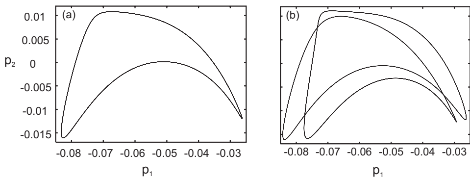
Figure 19. Two-dimensional projections of the phase portraits of the limit cycles found to the left side on branch II when \sigma_2 = (a) 0.744328 (p-1), \sigma_2 = (b) 0.7429668 (p-2).
