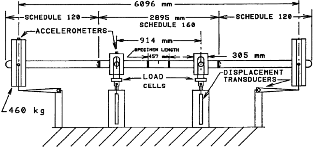
Figure 12: Schematics of the experiment 1.1-3 (Wilkowski, Schmidt, & Scott, 1997).
