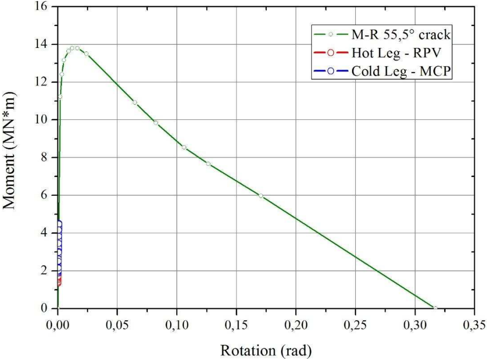
Figure 15: Moment vs Rotations for a 55.5° crack.
