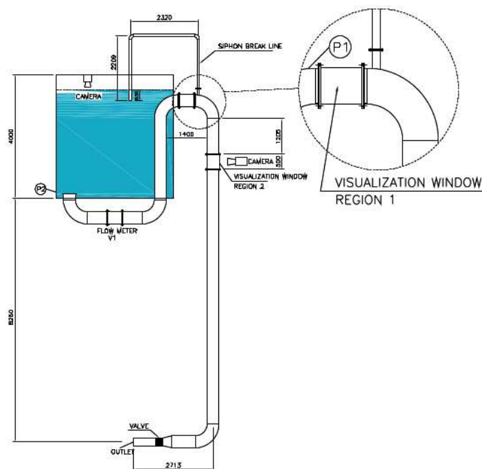
Figure 1: View of the test geometry with the main constructive parameters (Courtesy of Seo et al. (2012)).
