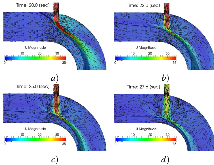
Figure 9: Velocity magnitude and vectors over the symmetry plane around the siphon discharge at four times. a): 20 sec. b): 22 sec. c): 25 sec. d): 27.6 sec
