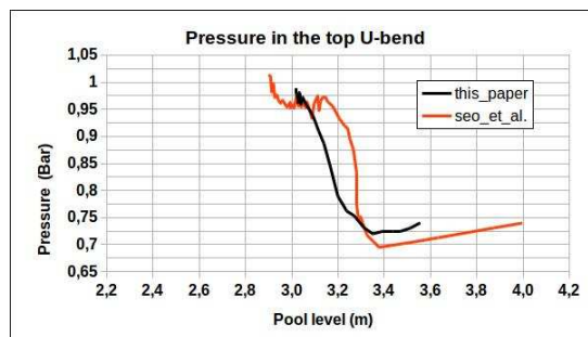
Figure 7: Pressure in the top U-bend. Comparison with the numerical results (Euler-Euler model) from Seo et al. (2012)
