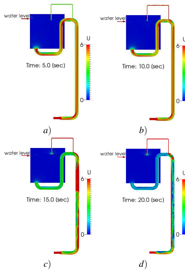
Figure 8: Velocity U over the symmetry plane at four times. a): 5 sec. b): 10 sec. c): 15 sec. d): 20 sec
