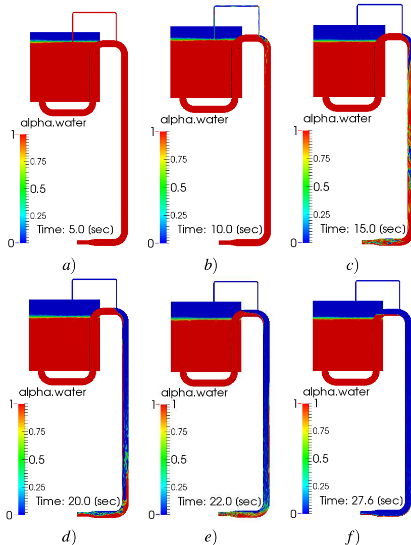
Figure 4: Volume fraction of water over the symmetry plane at six times. a): 5 sec. b): 10 sec. c): 15 sec. d): 20 sec e): 22 sec. f): 27.6 sec.
