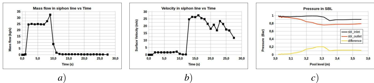
Figure 6: Flow through the SBL. a): Mass flow vs. time b): Velocity vs. time. c): Pressures in the SBL vs pool level
