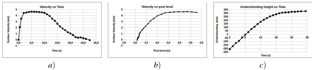
Figure 5: a): Surface velocity in the main line vs time. b): Surface velocity in the main line vs pool height. c) Undershooting vs time
