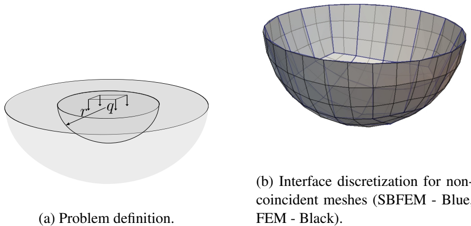
Figure 2: Settlement problem.
